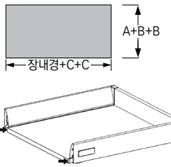
6. Front panel
